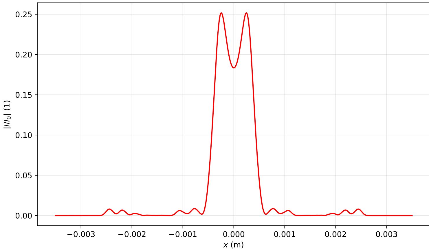
Intensity profile I(x, y = 0, z = 1.751)/I_0 , P_{in}=5.0P_{cr} , artificial time
